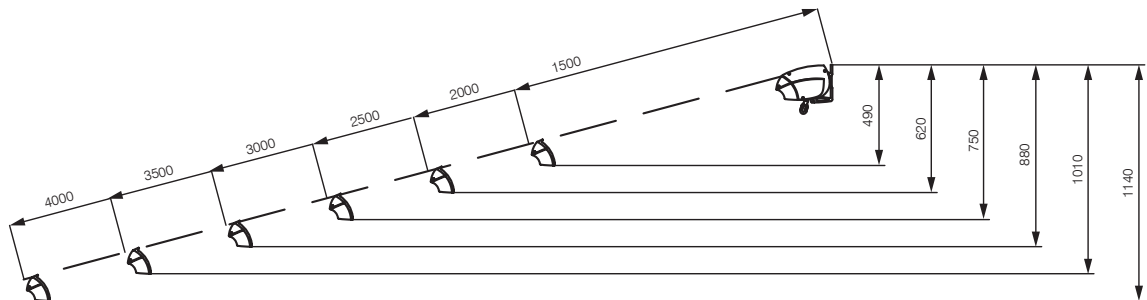
System height for standard 15° slope
