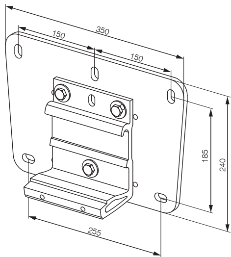
Bracket spreader plate
